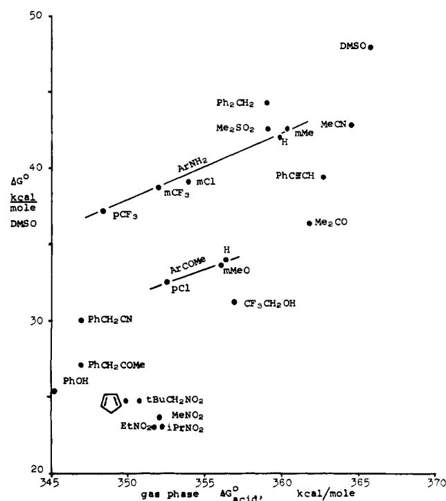
Figure 4. Plot of gas-phase acidities vs. acidities in Me 2 SO (DMSO). Data are from Table VI.
