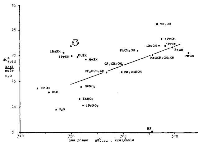
Figure 3. Plot of gas-phase acidities vs. aqueous acidities. Data are from Table VI. The line is for F 3 CCH 2 OH, F 2 CHCH 2 OH, MeOCH 2 CH 2 OH, and EtOH.
