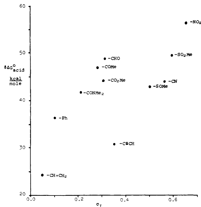
Figure 1. Gas-phase acidities of \text{CH}_3\text{EWG} vs. \sigma_I(\text{EWG}) . Data are from Table III.
