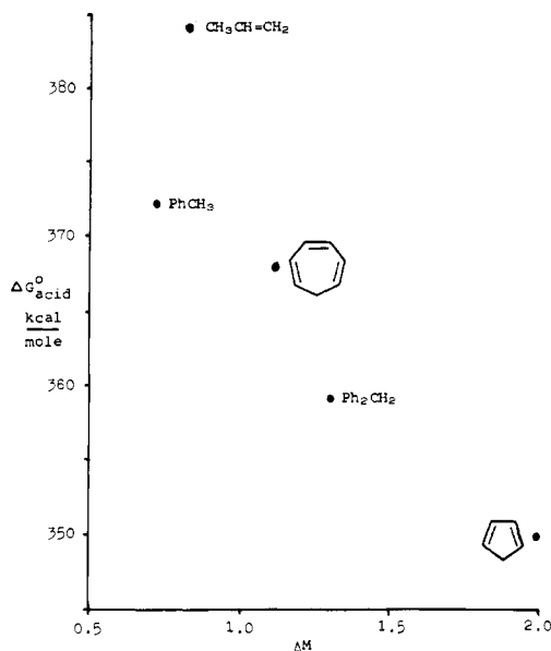
Figure 5. Gas-phase acidities of hydrocarbons vs. \Delta M for delocalization.
