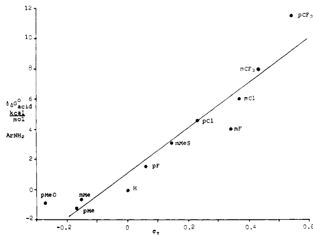
Figure 2. Hammett correlation of gas-phase acidities of anilines vs. \sigma_1 .
