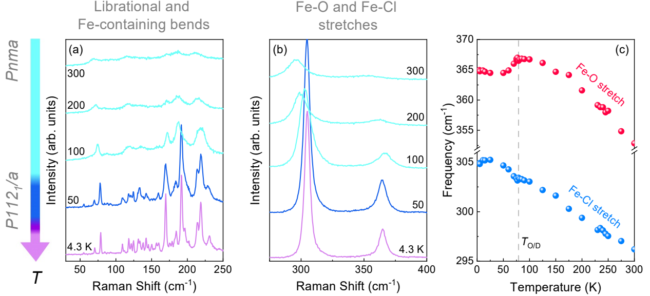
Figure 4: Variable temperature Raman scattering response of (\text{NH}_4)_2\text{FeCl}_5\cdot\text{H}_2\text{O} across the order-disorder transition highlighting the (a) low frequency \text{NH}_4 librations, the Cl-Fe-Cl and Cl-Fe-O bending modes, and (b) the Fe-Cl and Fe-O stretching modes. (c) Frequency vs. temperature plot emphasizing changes across T_{\text{O/D}} = 79 K. Ordering of the ammonium ion begins at 79 K and continues until approximately 50 K, creating a wide dynamic range for the ordering process. These data were collected at ambient pressure.
