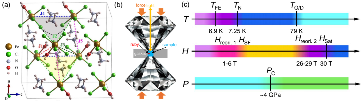
Figure 1: (a) Crystal structure of (\text{NH}_4)_2\text{FeCl}_5 \cdot \text{H}_2\text{O} at 300 K showing the five different magnetic exchange interactions ( J_{1-5} ). 31–33 The latter are represented with colored dashed lines and are formed by intermolecular hydrogen and halogen bonding . The [\text{FeCl}_5 \cdot \text{H}_2\text{O}]^{2-} clusters create a herringbone-like chain down the b -axis with \text{NH}_4^+ ions in symmetrically equivalent positions to balance charge. (b) Schematic representation of the diamond anvil cell used for high pressure vibrational spectroscopy. (c) Schematic summarizing the temperature-, magnetic field-, and pressure-induced transitions uncovered in this system thus far.
