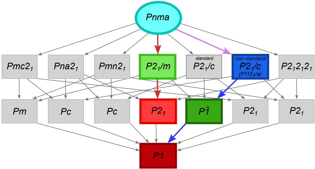
Figure 6: Schematic representation of the symmetry tree for (\text{NH}_4)_2\text{FeCl}_5 \cdot \text{H}_2\text{O} . 58-60 Here, Pnma is the high temperature space group. P112_1/a , which is a non-standard subset of P2_1/c , is the low temperature space group. The high to low temperature phase transition is indicated by the purple arrow. Both can be driven to lower symmetry with pressure. Their sequential pathways are highlighted in red and blue, respectively.
