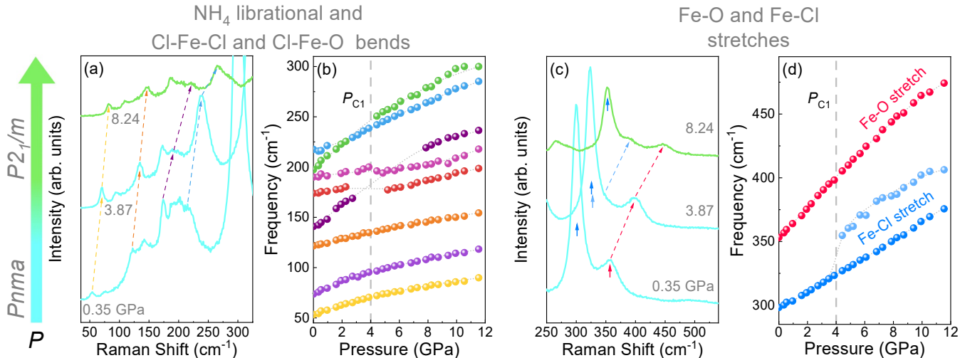
Figure 2: Close-up view of the Raman scattering response of (\text{NH}_4)_2\text{FeCl}_5\cdot\text{H}_2\text{O} as a function of pressure at 300 K for (a) the \text{NH}_4 librations and the Cl-Fe-Cl and Cl-Fe-O bending modes as well as (c) the Fe-Cl stretching and Fe-O stretching modes. Splitting of the Fe-Cl stretch is an excellent signature of the 4 GPa structural phase transition ( P_{C,1} ). The arrows guide the eye. (b,d) Frequency vs. pressure data for these data. Dotted lines guide the eye in panel (b). Error bars are on the order of the symbol size.
