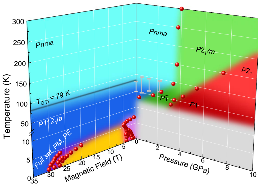
Figure 7: P - T - H phase diagram of multiferroic (\text{NH}_4)_2\text{FeCl}_5 \cdot \text{H}_2\text{O} . The space groups are labeled. Extrapolating P_{C,2} to room temperature, we expect to find the polar + chiral P2_1 phase just above 15 GPa. As shown by the gray bars, \partial T_{o/d}/\partial P is slightly positive as discussed in Supporting information . The gray areas on the phase diagram are inaccessible in our experiments.
