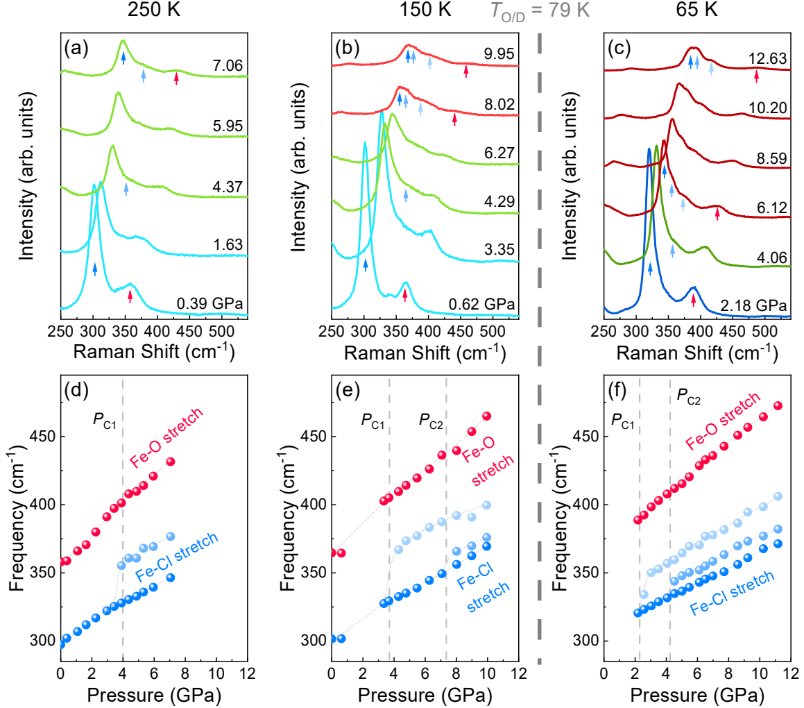
Figure 5: Close-up view of the Raman-active Fe-Cl and Fe-OH 2 stretching modes as a function of pressure. (a,b) Spectra taken above the order-disorder temperature at 250 and 150 K and (d,e) their corresponding frequency vs. pressure plots. (c,f) Raman spectra collected at 65 K and the corresponding frequency vs. pressure trends. The latter is below the 79 K order-disorder transition.
