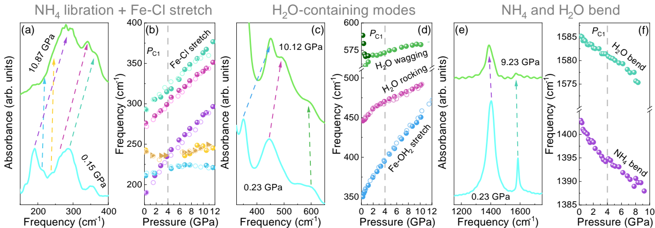
Figure 3: Close-up view of the infrared absorbance of (\text{NH}_4)_2\text{FeCl}_5\cdot\text{H}_2\text{O} as a function of pressure at 300 K for (a) the low frequency libration modes and the Fe-Cl stretch, (c) the H 2 O-containing modes, and (e) the NH 4 and H 2 O bending modes. (b,d,f) Frequency vs. pressure trends for these regions. Closed and open symbols in the frequency vs. pressure plots are from two independent runs.
